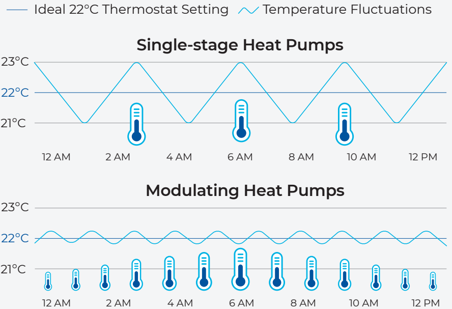
Figure 2: Single-stage vs. Modulating
